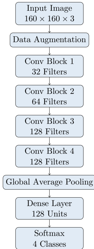
Figure 2: Architecture of the custom CNN baseline
