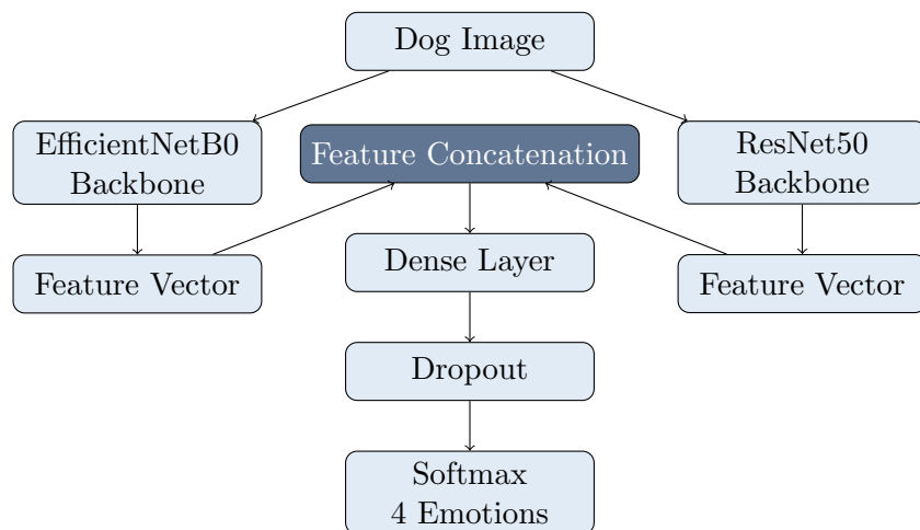
Figure 3: Feature-level EfficientNetB0 + ResNet50 ensemble
